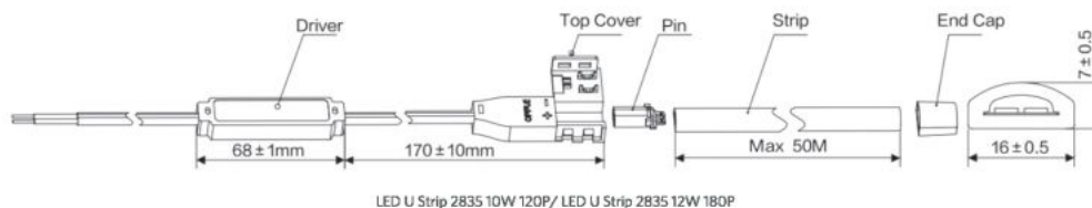
LEDStrip-U 50M-2835-Accessory Bag
