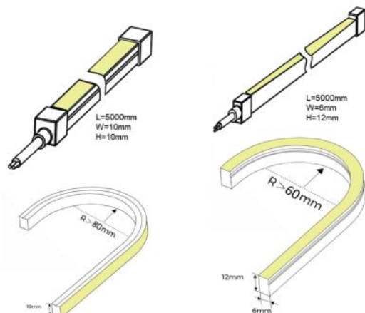
LED-24/10-2835-120NH(0612S)
