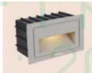
AT-21 COB 3W - IP54 L105 x W50 x H58 Ø L95 x W50 x H53 390.000đ
